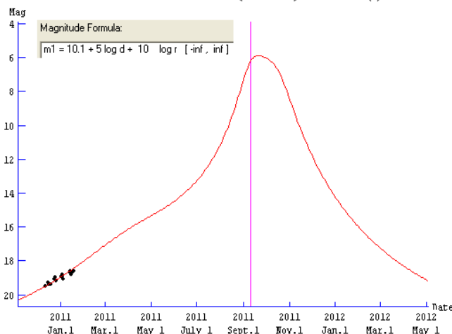
C/2010 X1 (Elenin)
